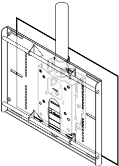
PSD-D 1-1/2" NPT Ceiling Adapter (Dual Side)
