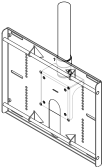
PSD-S 1-1/2" NPT Ceiling Adapter (Single Side)
