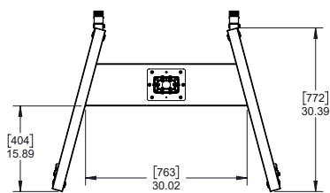
SECTION A-A CART BASE DETAIL
