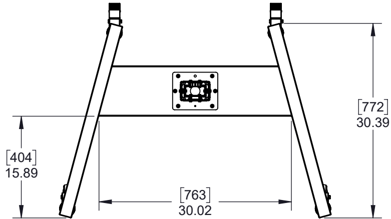
SECTION A-A CART BASE DETAIL
