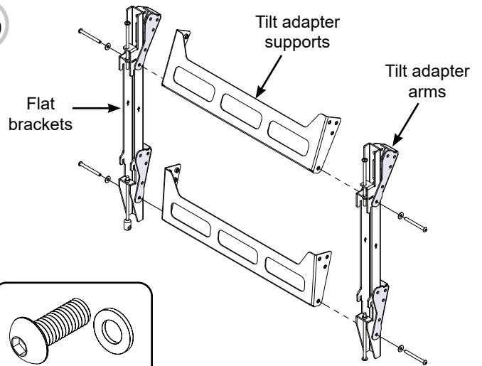
1/4-20" x 3/4" & washers
