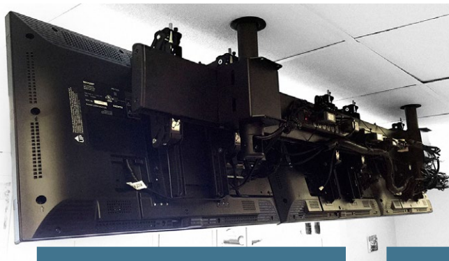
UNISTRUT CHANNEL ADAPTER MOUNTS
