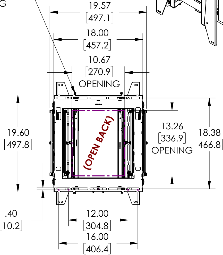
(SERVICE POSITION)
