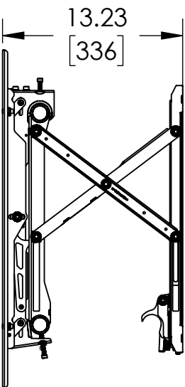
(FULLY EXTENDED)
