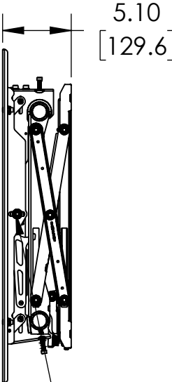
(FULLY COLLAPSED)
