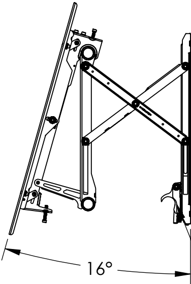
(SERVICE POSITION)
