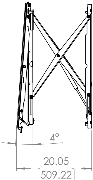
(SERVICE POSITION)
