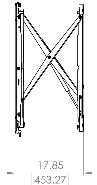
(FULLY EXTENDED)
