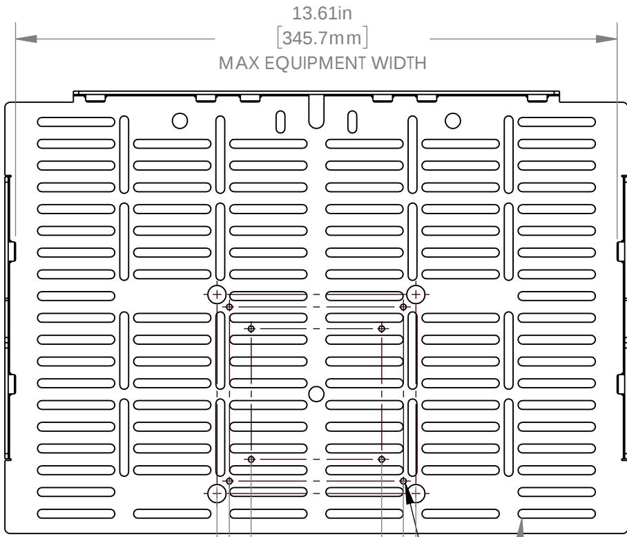
VESA 75X75 VESA 100X100 4.50in [114.3mm] M4 X 0.7 TAP 8 PLACES
