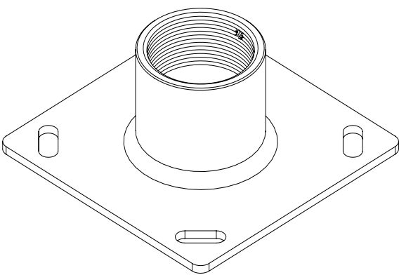
PP-6 CEILING ADAPTER
