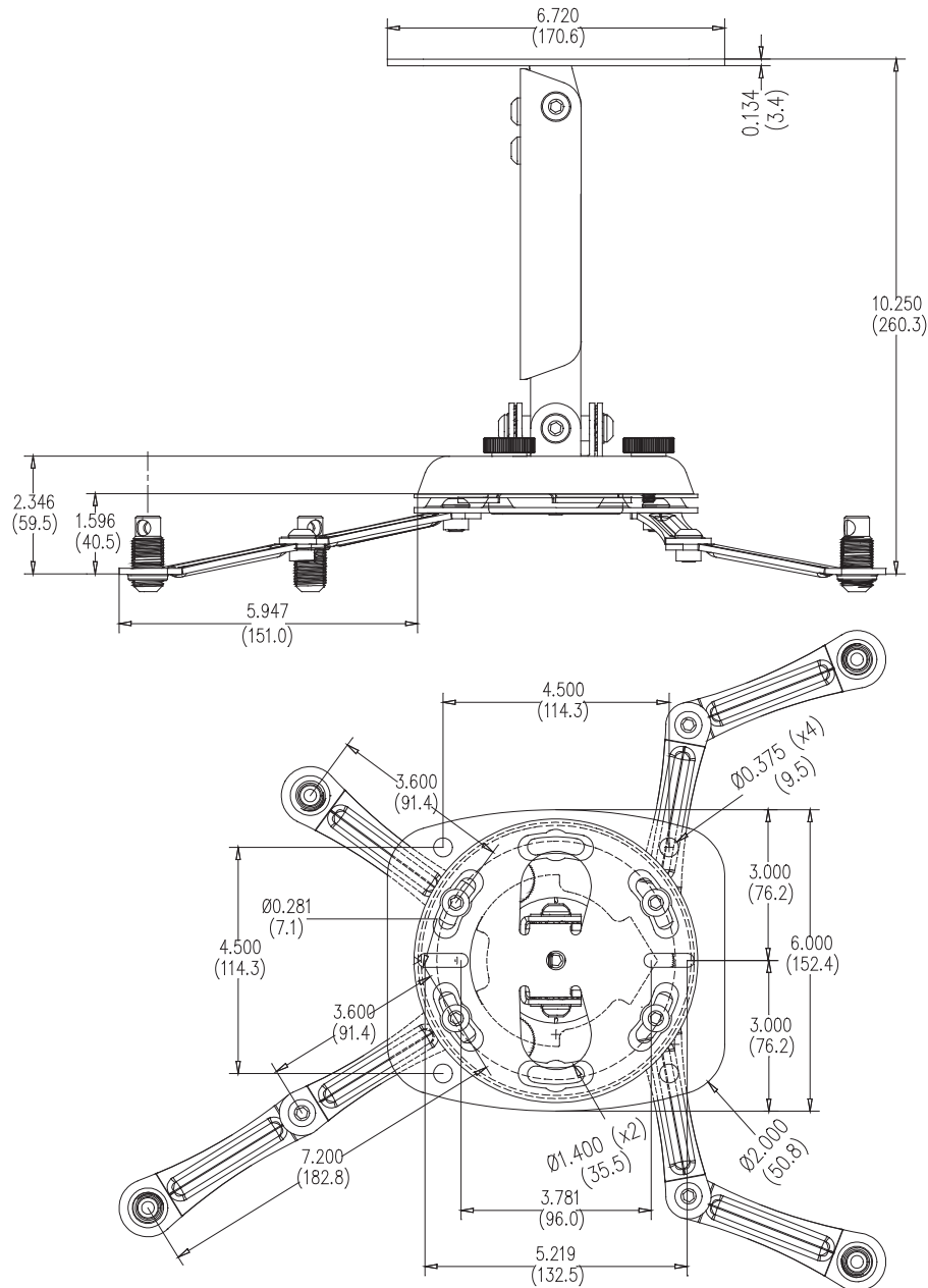
Figure 9. Technical Dimensions
