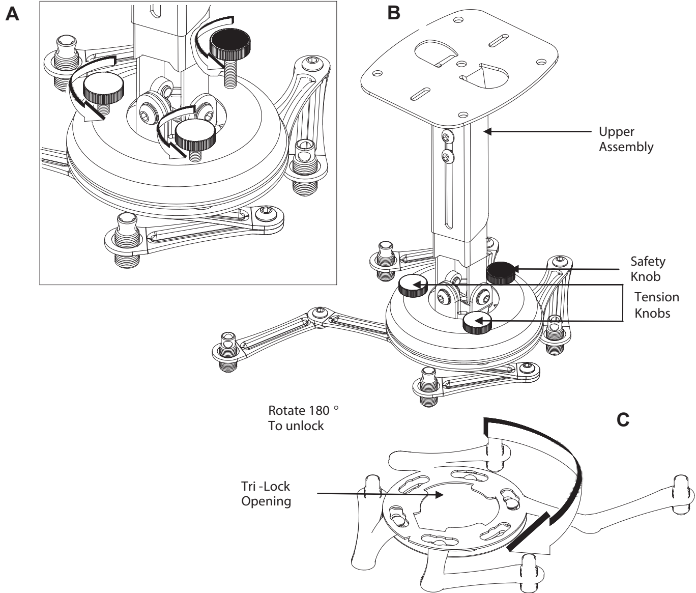
Figure 2. Mount Preparation
