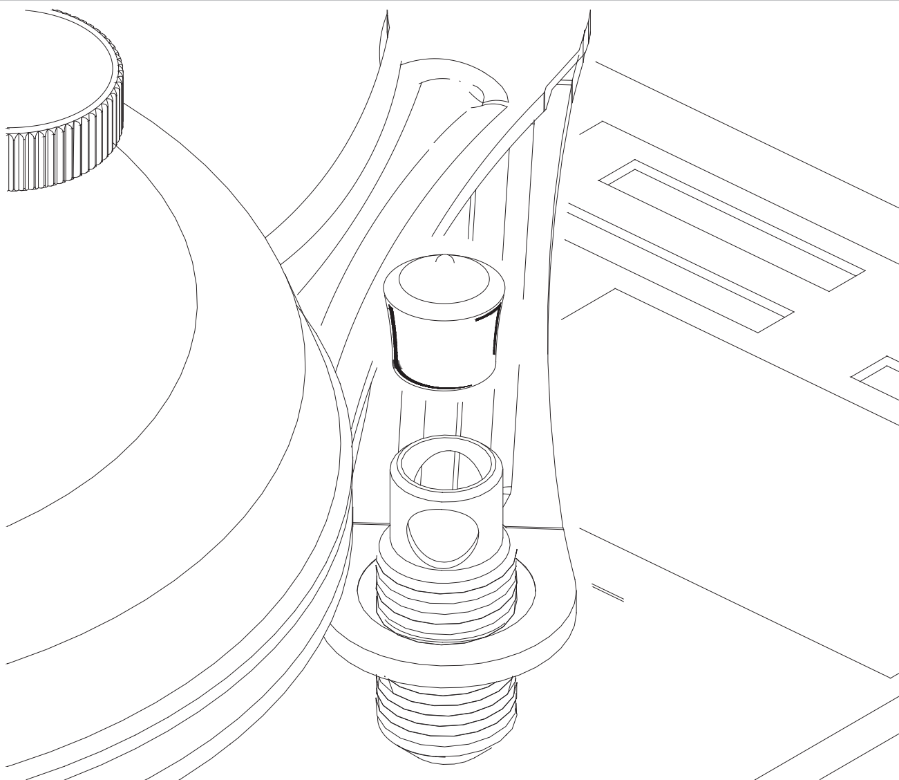
Figure 8. Plastic Cap Installation
