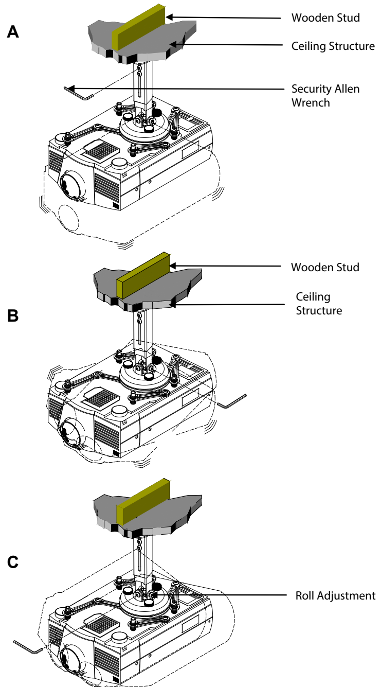
Figure 7. Final Adjustments
