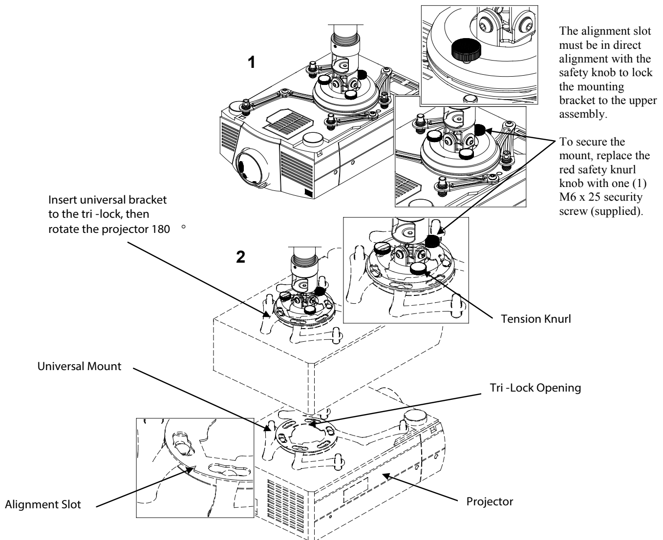
Figure 6. Low Profile Installation
