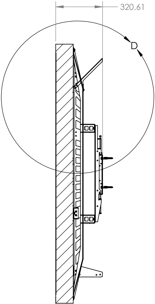
SECTION C-C
