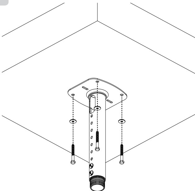
5/16" X 3" LAG BOLT
