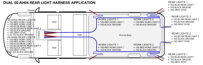
DUAL 00-AH04 REAR LIGHT HARNESS APPLICATION
