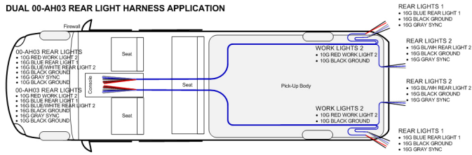
DUAL 00-AH03 REAR LIGHT HARNESS APPLICATION
