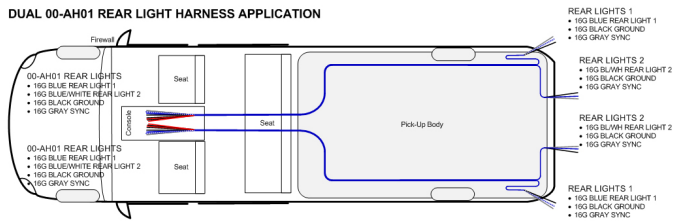
DUAL 00-AH01 REAR LIGHT HARNESS APPLICATION
