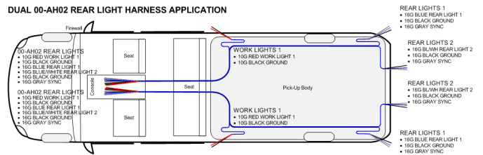
DUAL 00-AH02 REAR LIGHT HARNESS APPLICATION
