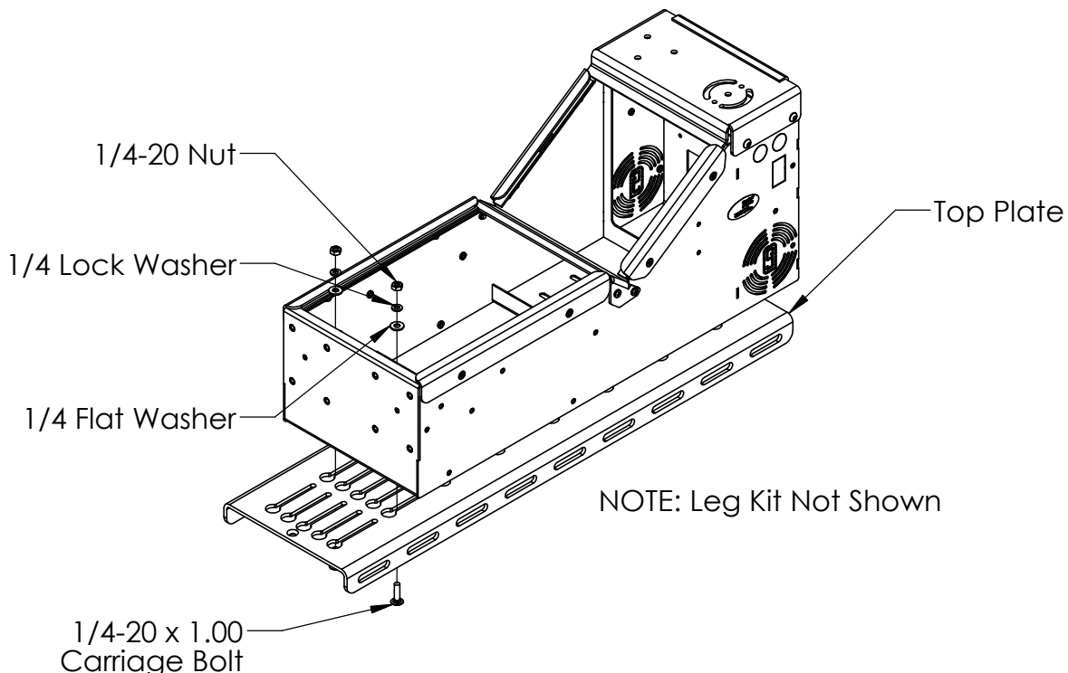
FIG 1 - Console Installation on Top Plate
