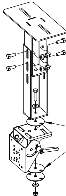
12" - 15" CONFIGURATION
