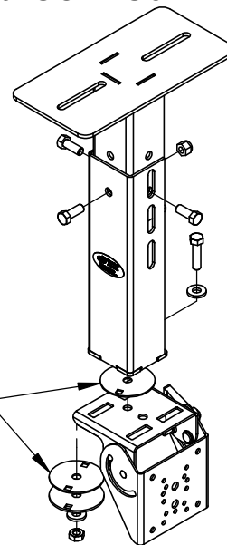
16" CONFIGURATION
