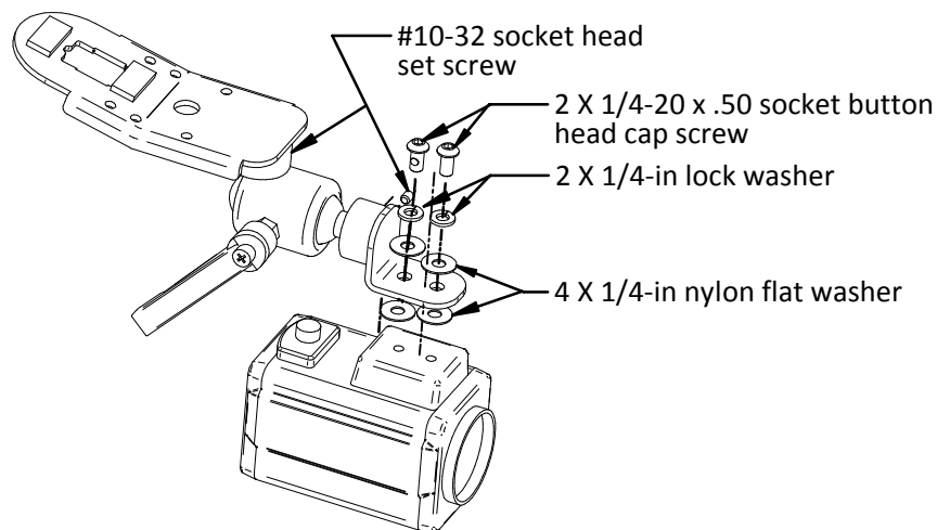
Figure 2: Assemble camera with 1/4-in fasteners
