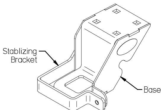
FIG. 1 Isometric Top View
