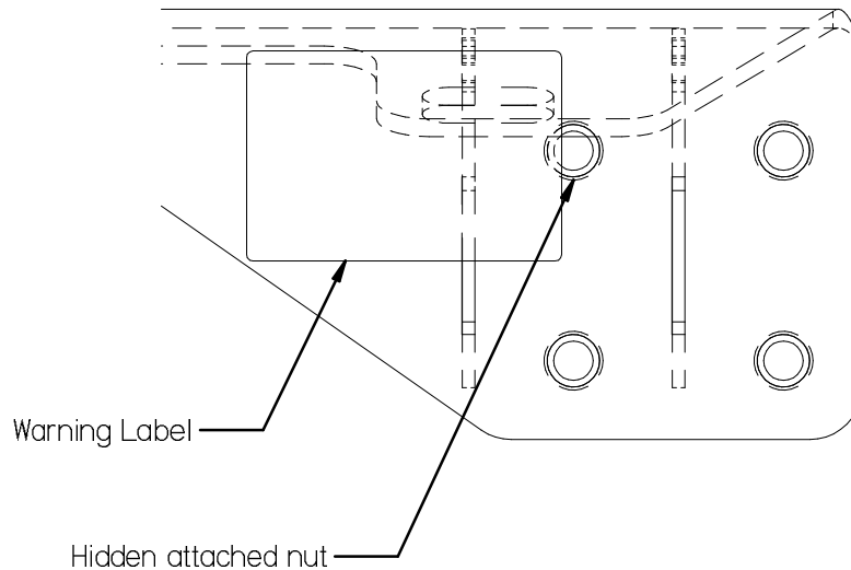
Fig. 2 Placement of the product warning label
